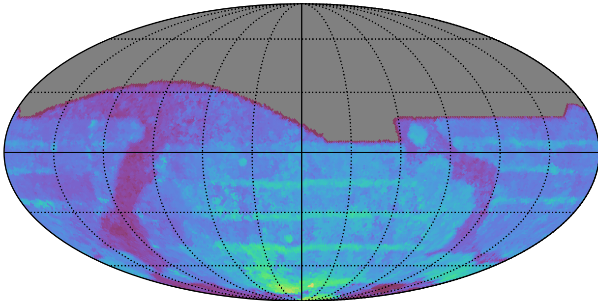
too_10_1v3.4_10yrs All sky all bands: 80thPercentile Season Length
