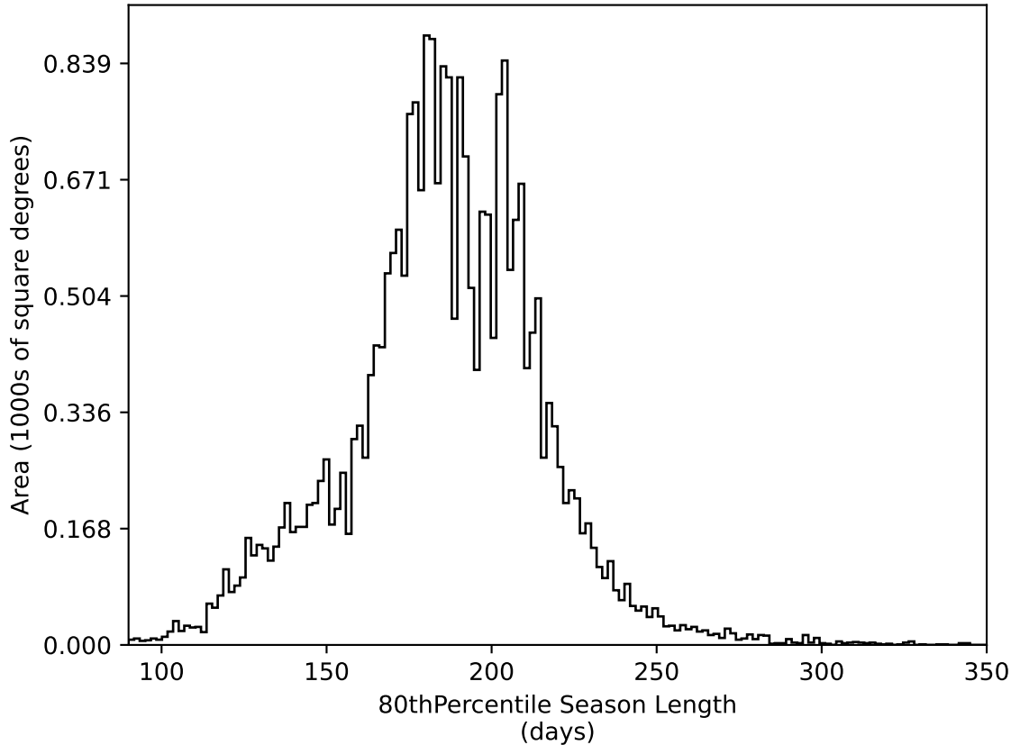
too_10_1v3.4_10yrs All sky all bands: 80thPercentile Season Length
