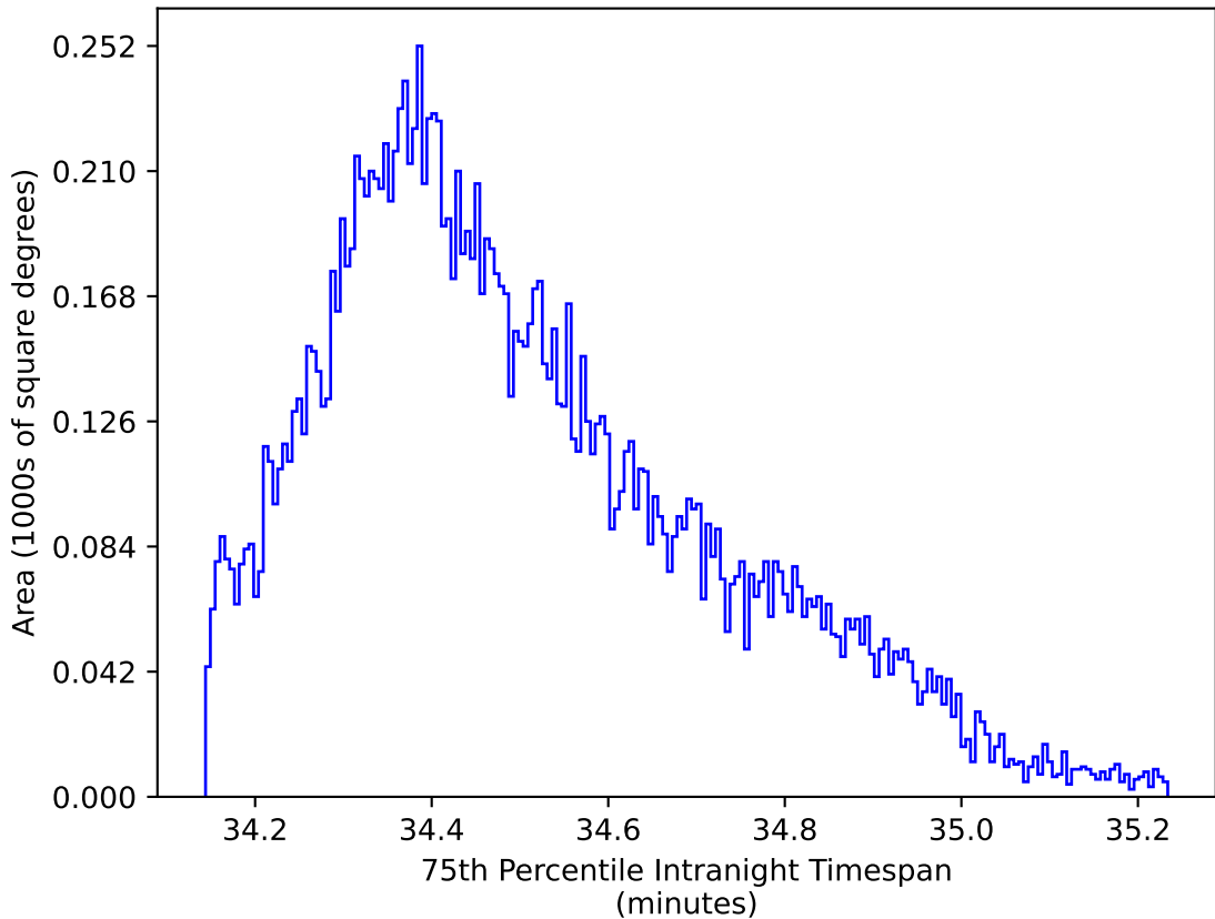
too_10_1v3.4_10yrs WFD zy bands: 75th Percentile Intranight Timespan
