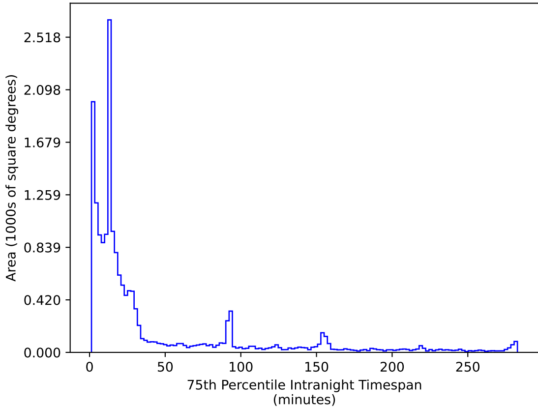
too_10_1v3.4_10yrs WFD r band: 75th Percentile Intranight Timespan
