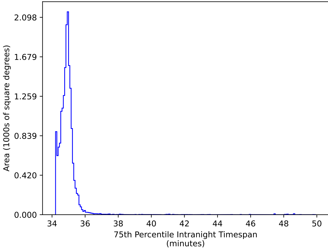
too_10_1v3.4_10yrs WFD iz bands: 75th Percentile Intranight Timespan
