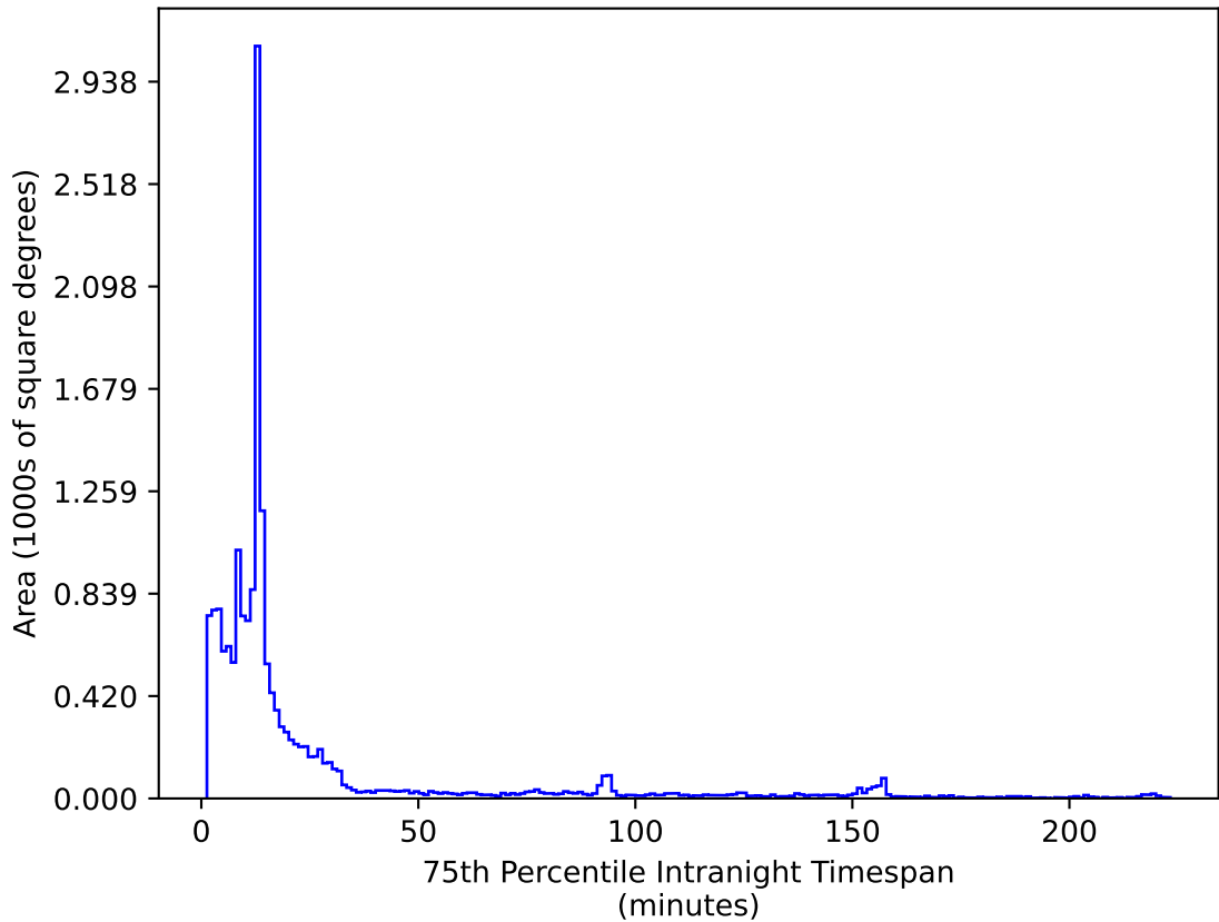
too_10_1v3.4_10yrs WFD i band: 75th Percentile Intranight Timespan
