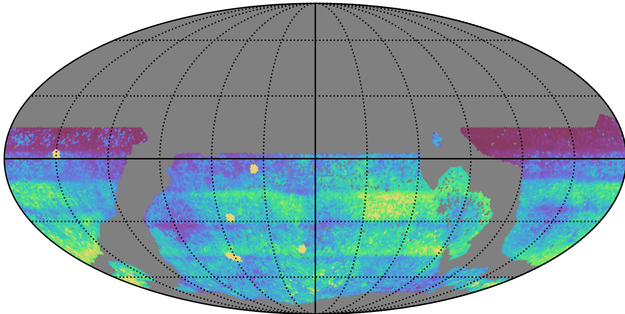
too_10_1v3.4_10yrs WFD: 75th Percentile Intranight Timespan
