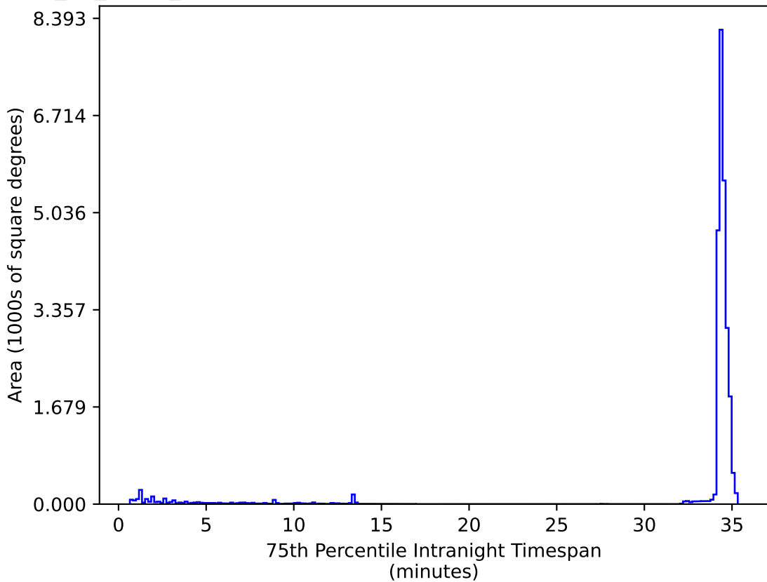
too_10_1v3.4_10yrs All sky zy bands: 75th Percentile Intranight Timespan
