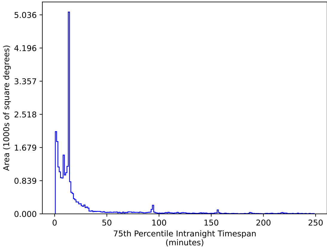
too_10_1v3.4_10yrs All sky z band: 75th Percentile Intranight Timespan
