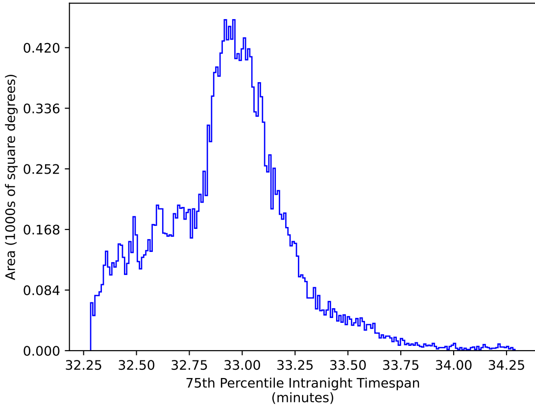
too_10_1v3.4_10yrs All sky y band: 75th Percentile Intranight Timespan
