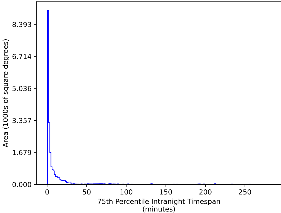
too_10_1v3.4_10yrs All sky u band: 75th Percentile Intranight Timespan
