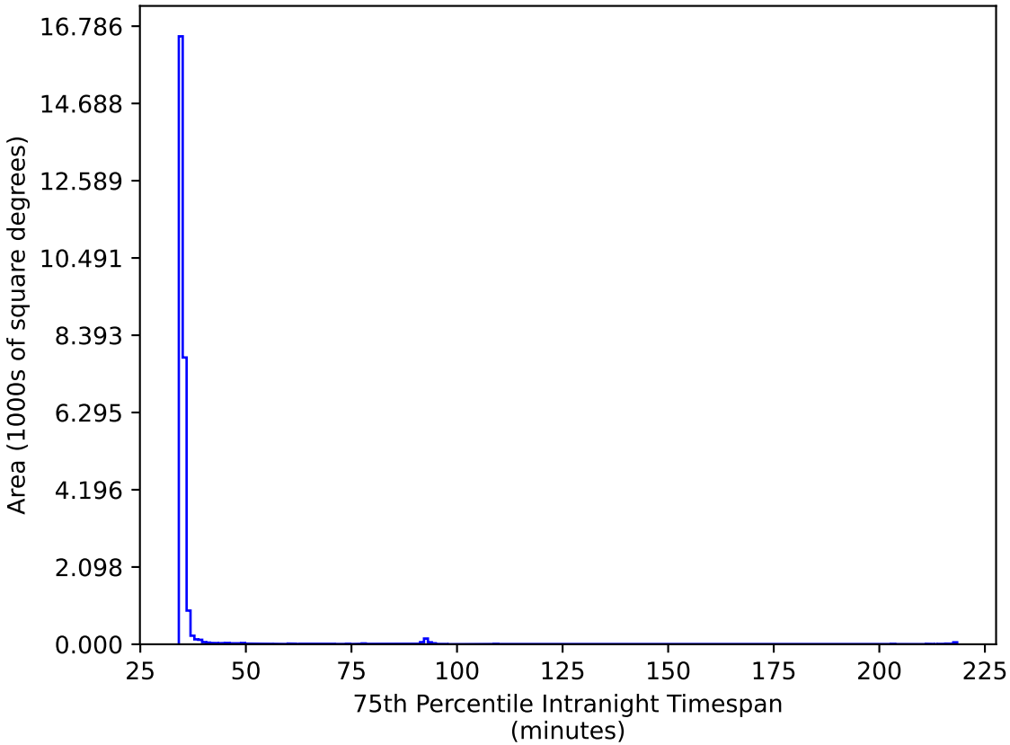
too_10_1v3.4_10yrs All sky ri bands: 75th Percentile Intranight Timespan
