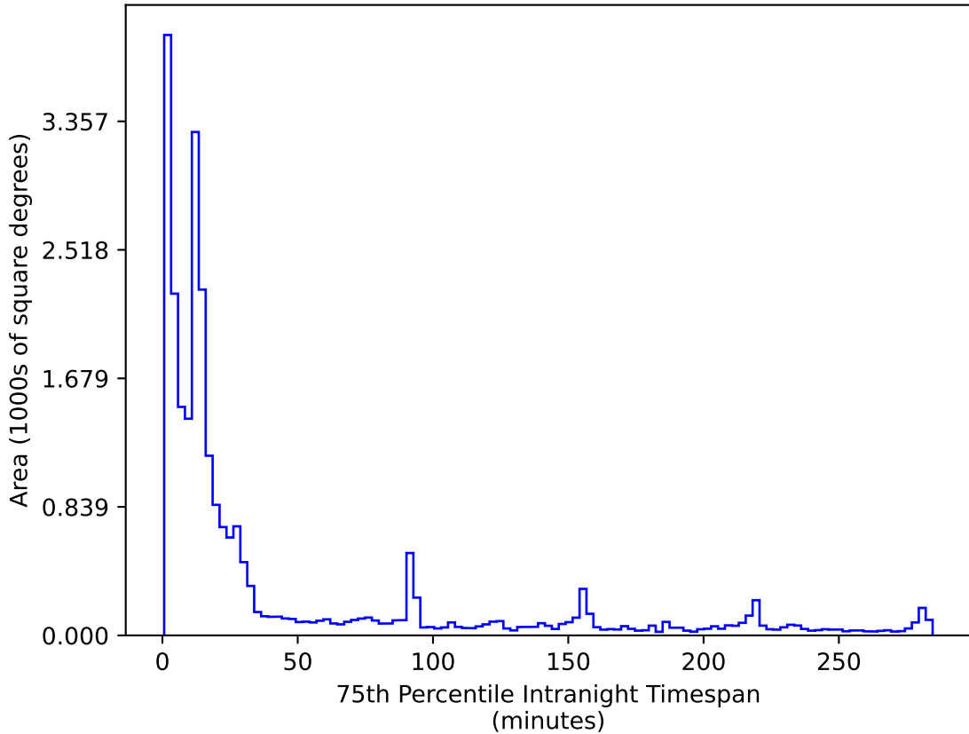
too_10_1v3.4_10yrs All sky r band: 75th Percentile Intranight Timespan
