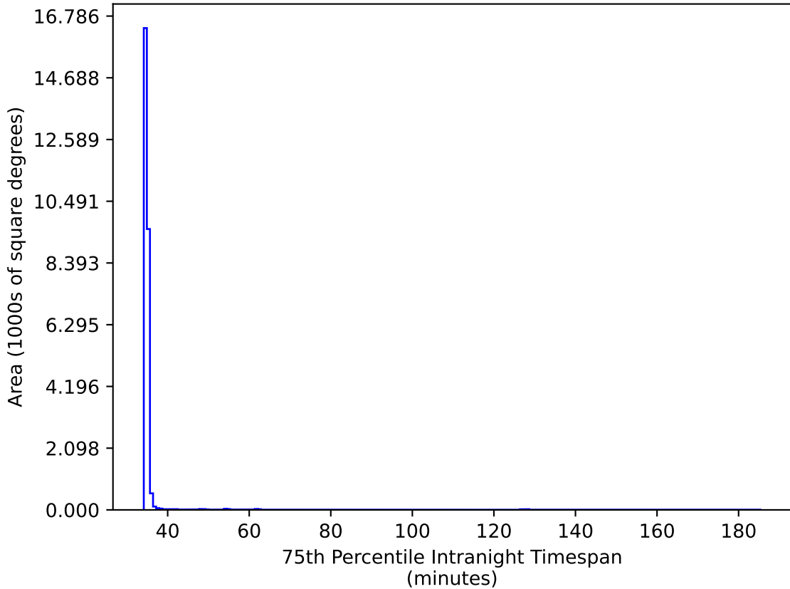
too_10_1v3.4_10yrs All sky iz bands: 75th Percentile Intranight Timespan
