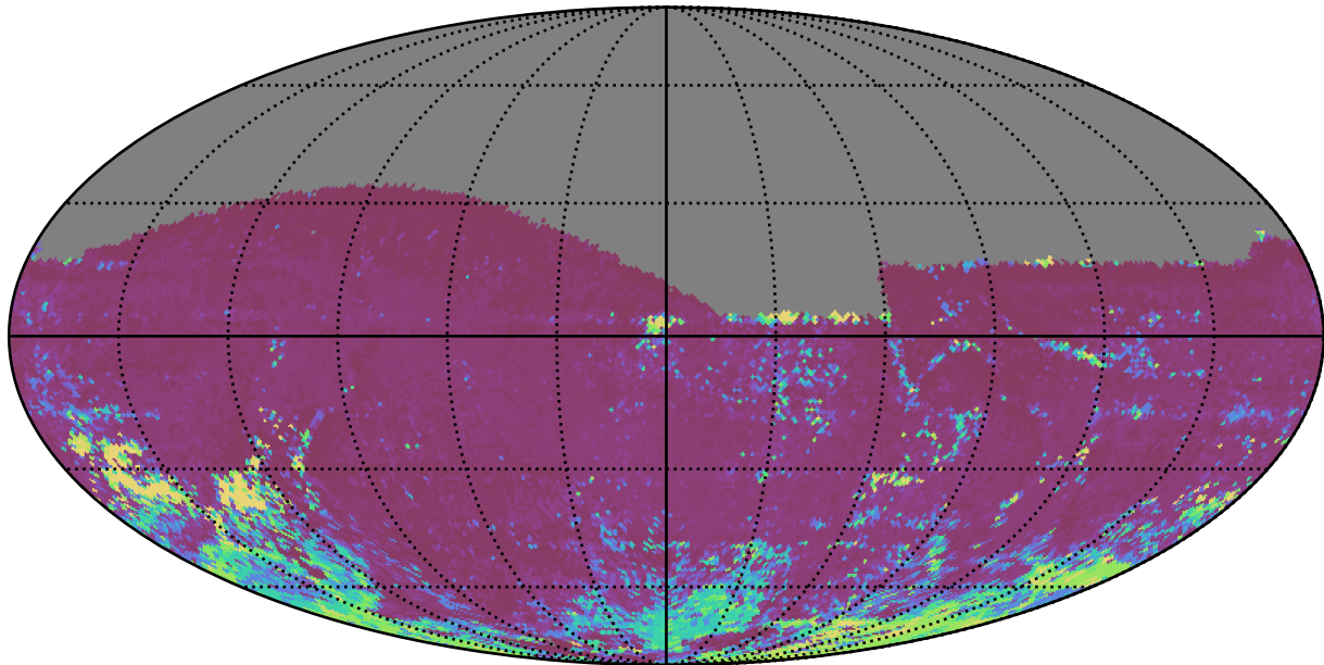
too_10_1v3.4_10yrs All sky i band: 75th Percentile Intranight Timespan
