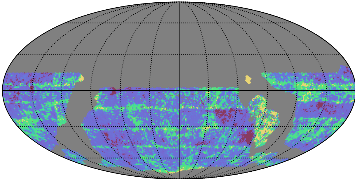
too_10_1v3.4_10yrs WFD z band: 20thPercentile Inter-Night Gap
