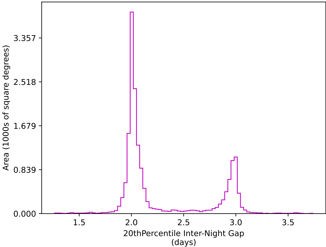
too_10_1v3.4_10yrs WFD z band: 20thPercentile Inter-Night Gap
