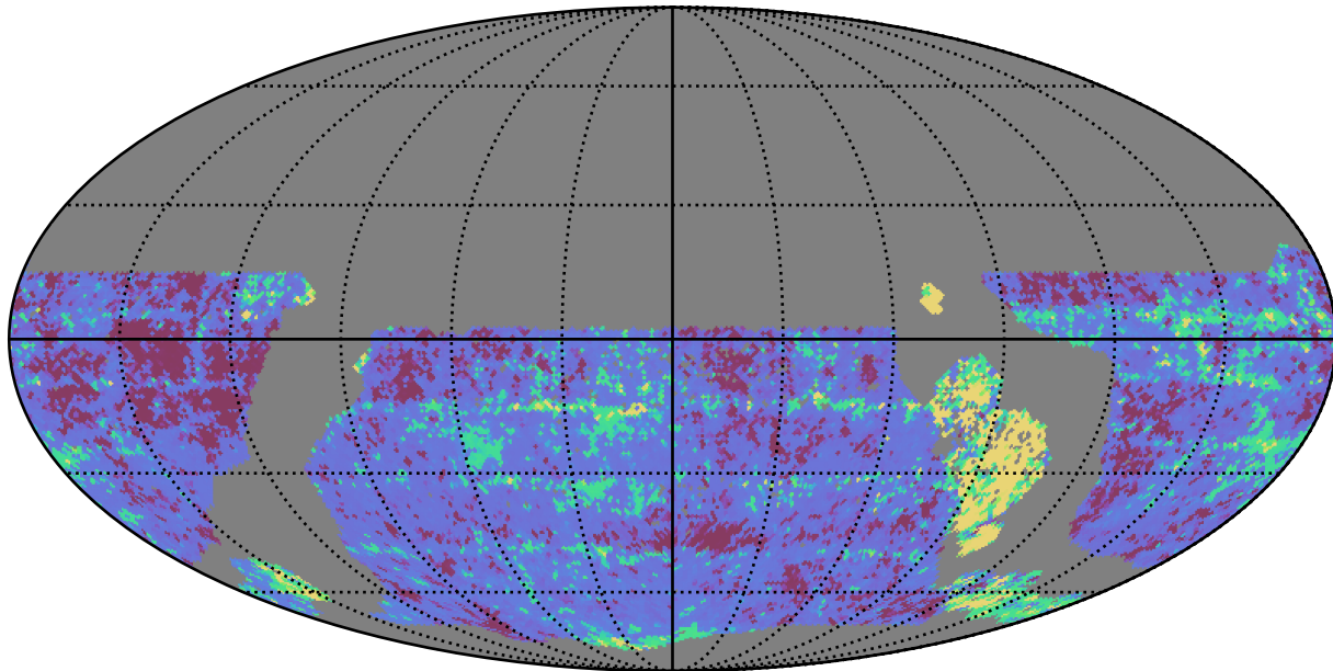
too_10_1v3.4_10yrs WFD y band: 20thPercentile Inter-Night Gap
