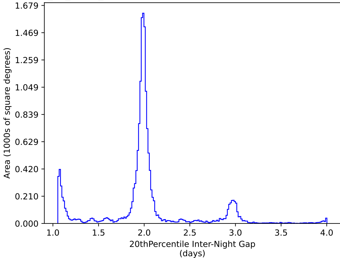
too_10_1v3.4_10yrs WFD y band: 20thPercentile Inter-Night Gap
