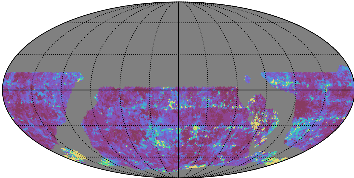
too_10_1v3.4_10yrs WFD u band: 20thPercentile Inter-Night Gap
