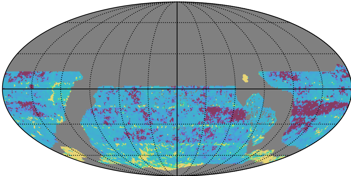
too_10_1v3.4_10yrs WFD r band: 20thPercentile Inter-Night Gap
