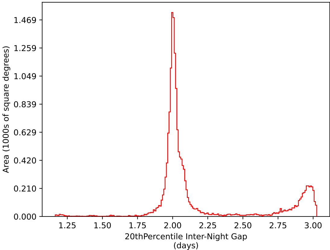
too_10_1v3.4_10yrs WFD i band: 20thPercentile Inter-Night Gap
