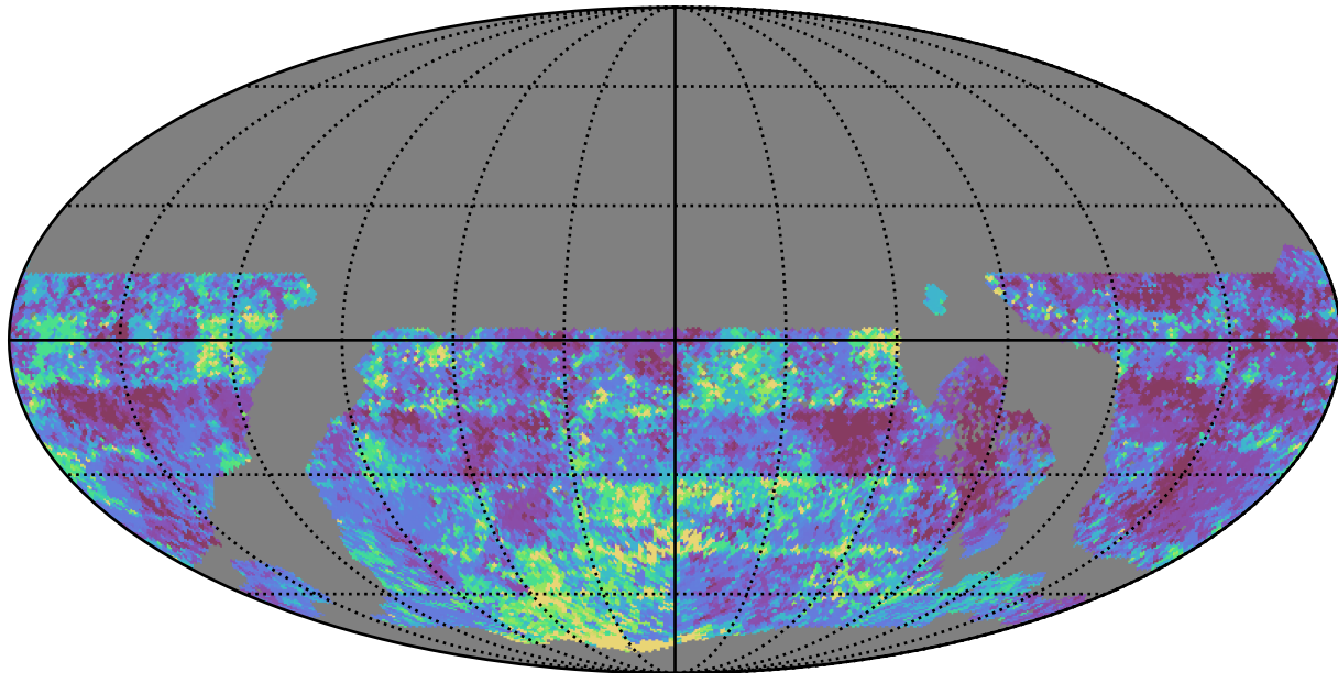
too_10_1v3.4_10yrs WFD g band: 20thPercentile Inter-Night Gap
