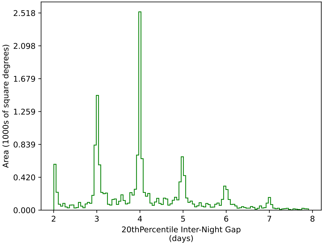
too_10_1v3.4_10yrs WFD g band: 20thPercentile Inter-Night Gap
