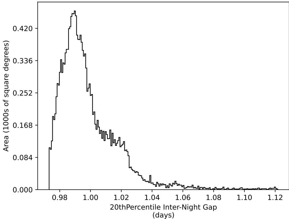
too_10_1v3.4_10yrs WFD all bands: 20thPercentile Inter-Night Gap
