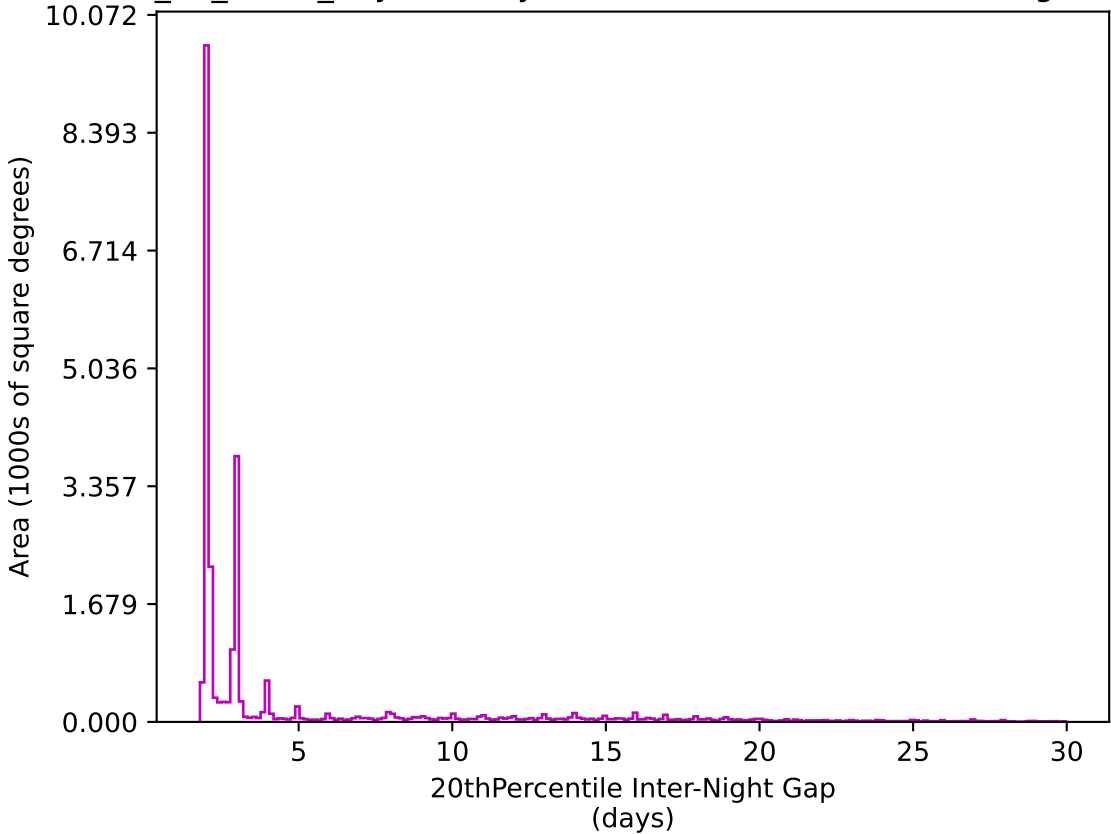
too_10_1v3.4_10yrs All sky z band: 20thPercentile Inter-Night Gap
