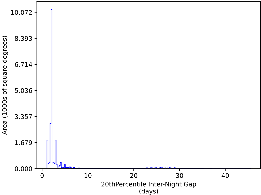
too_10_1v3.4_10yrs All sky y band: 20thPercentile Inter-Night Gap
