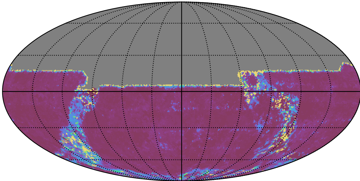
too_10_1v3.4_10yrs All sky u band: 20thPercentile Inter-Night Gap
