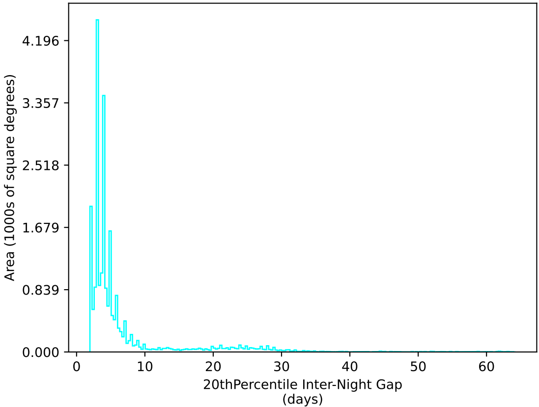
too_10_1v3.4_10yrs All sky u band: 20thPercentile Inter-Night Gap
