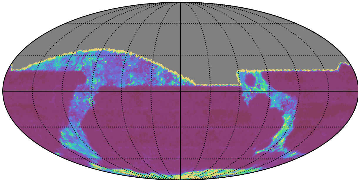
too_10_1v3.4_10yrs All sky r band: 20thPercentile Inter-Night Gap
