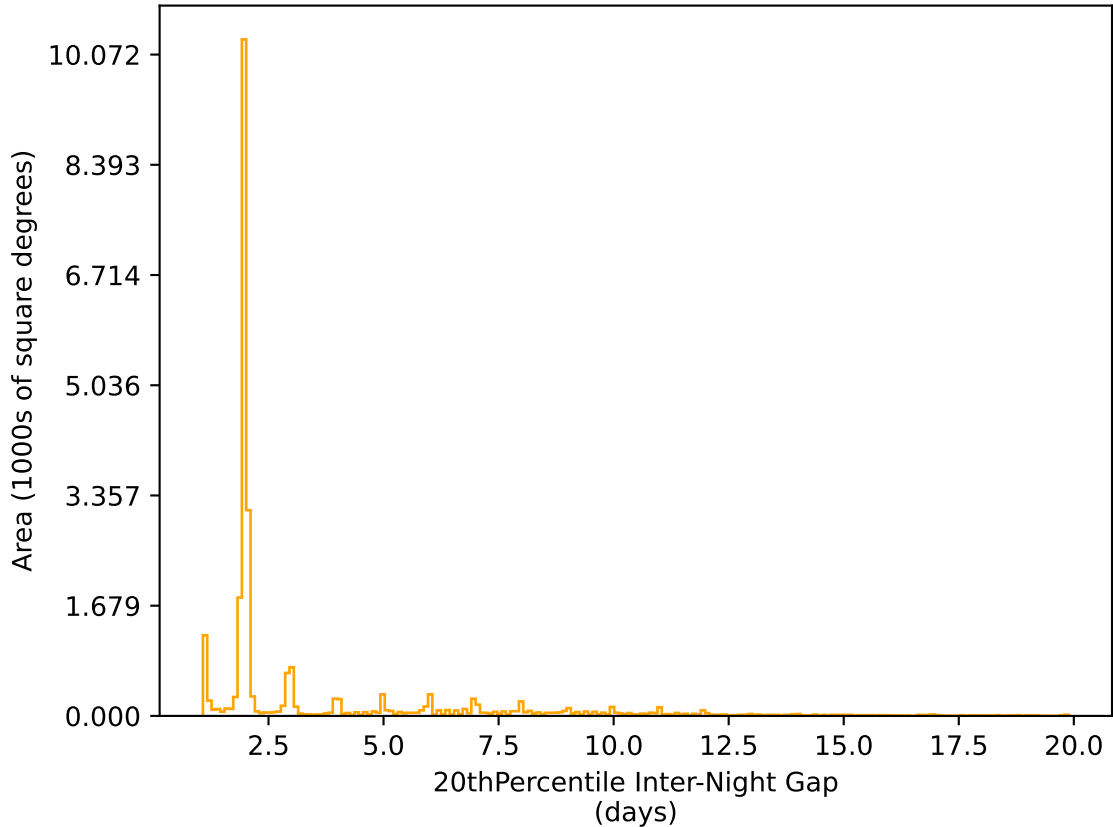
too_10_1v3.4_10yrs All sky r band: 20thPercentile Inter-Night Gap
