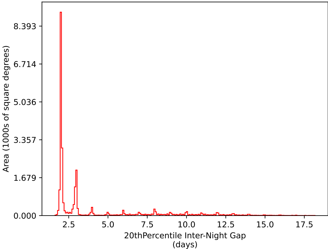
too_10_1v3.4_10yrs All sky i band: 20thPercentile Inter-Night Gap
