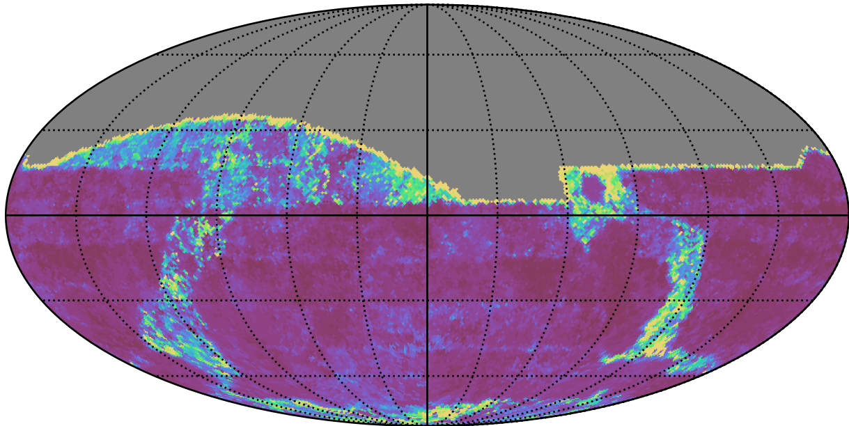
too_10_1v3.4_10yrs All sky g band: 20thPercentile Inter-Night Gap
