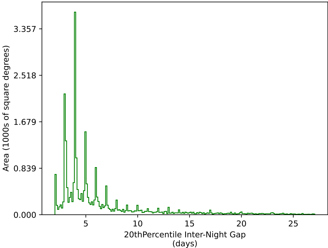
too_10_1v3.4_10yrs All sky g band: 20thPercentile Inter-Night Gap
