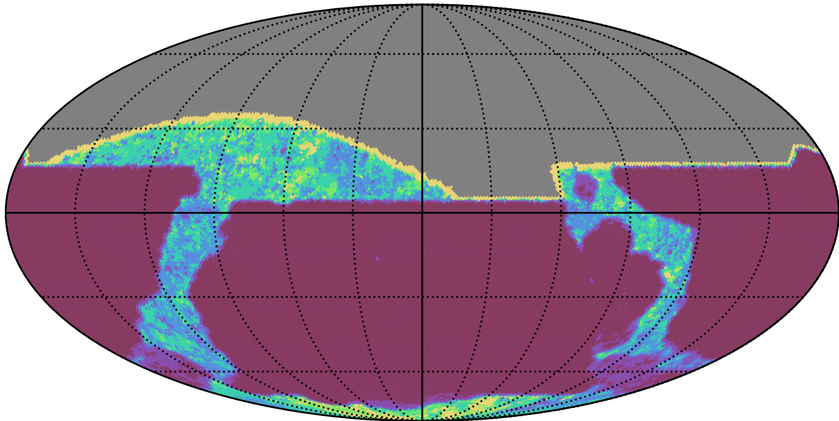
too_10_1v3.4_10yrs All sky all bands: 20thPercentile Inter-Night Gap
