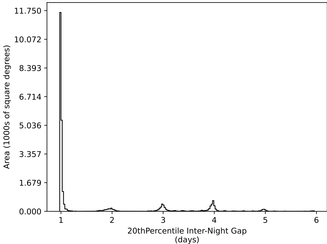
too_10_1v3.4_10yrs All sky all bands: 20thPercentile Inter-Night Gap
