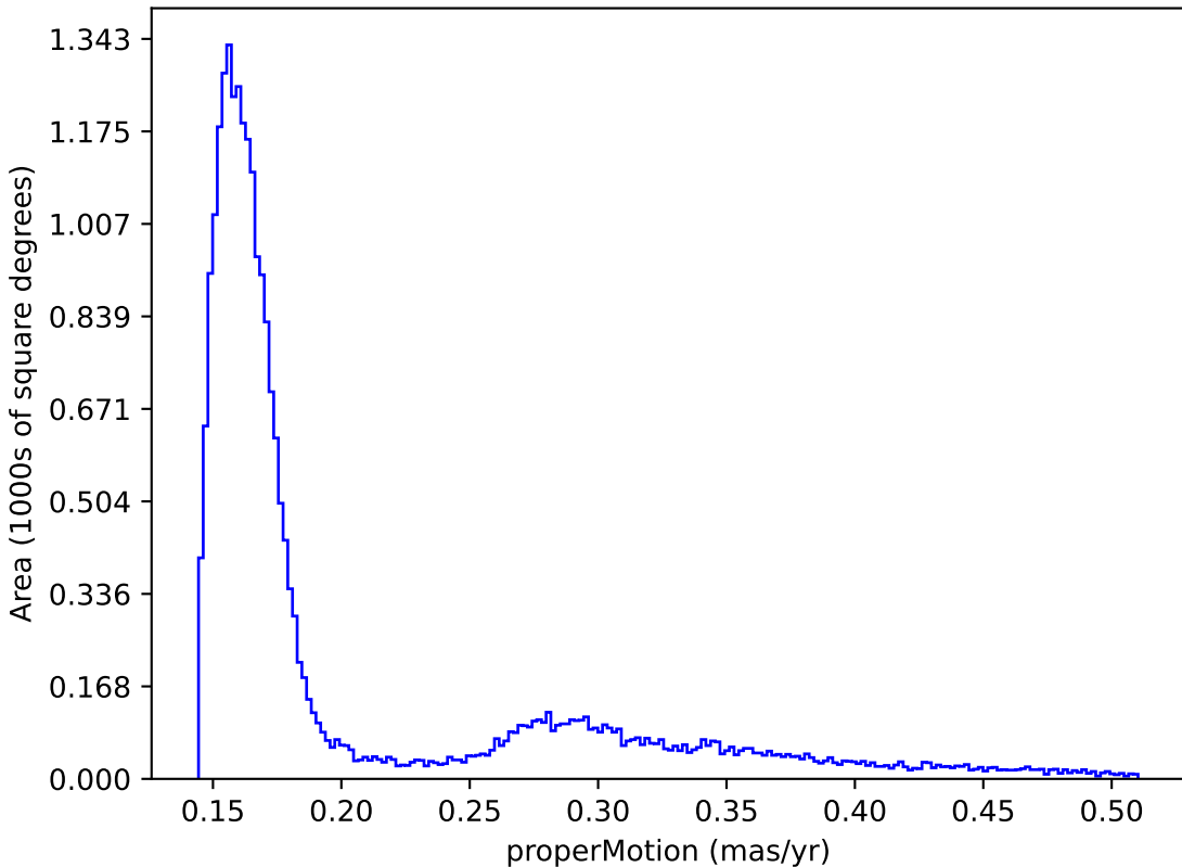
too_10_1v3.4_10yrs : properMotion
