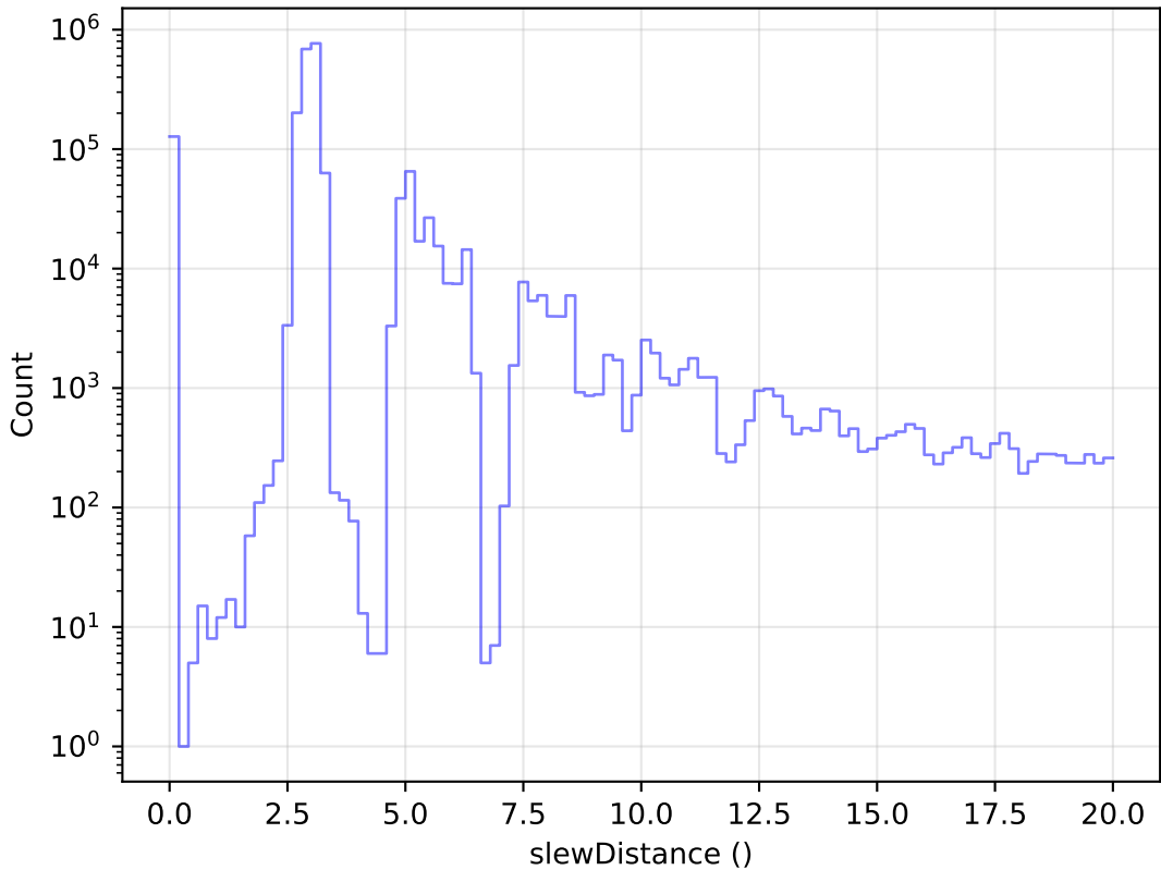
too_10_1v3.4_10yrs All visits: Zoom Slew Distance Histogram
