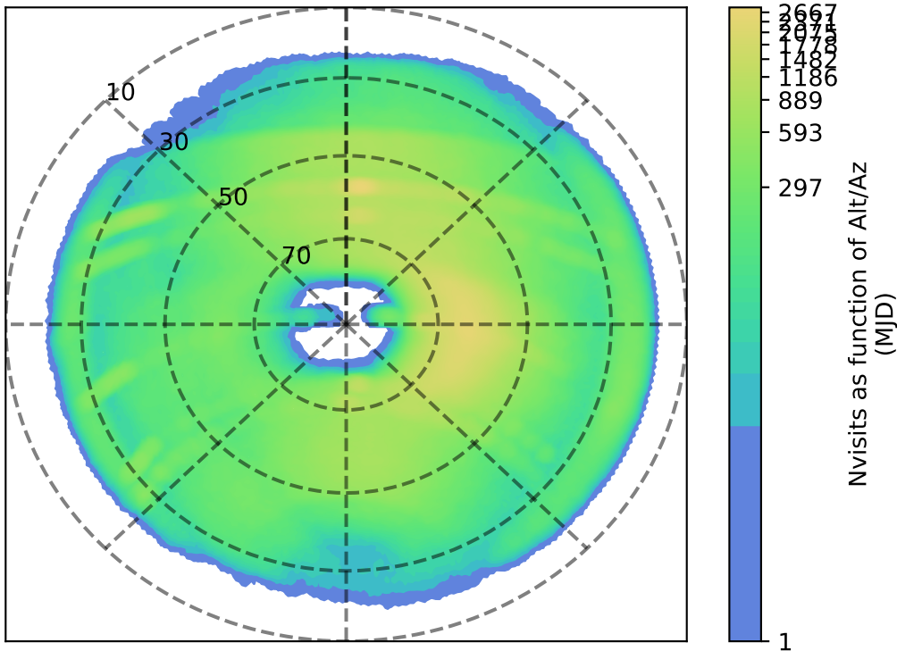
too_10_1v3.4_10yrs i: Nvisits as function of Alt/Az
