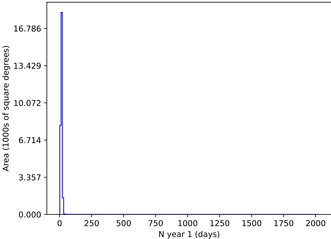
too_10_1v3.4_10yrs z and night < 365: N year 1
