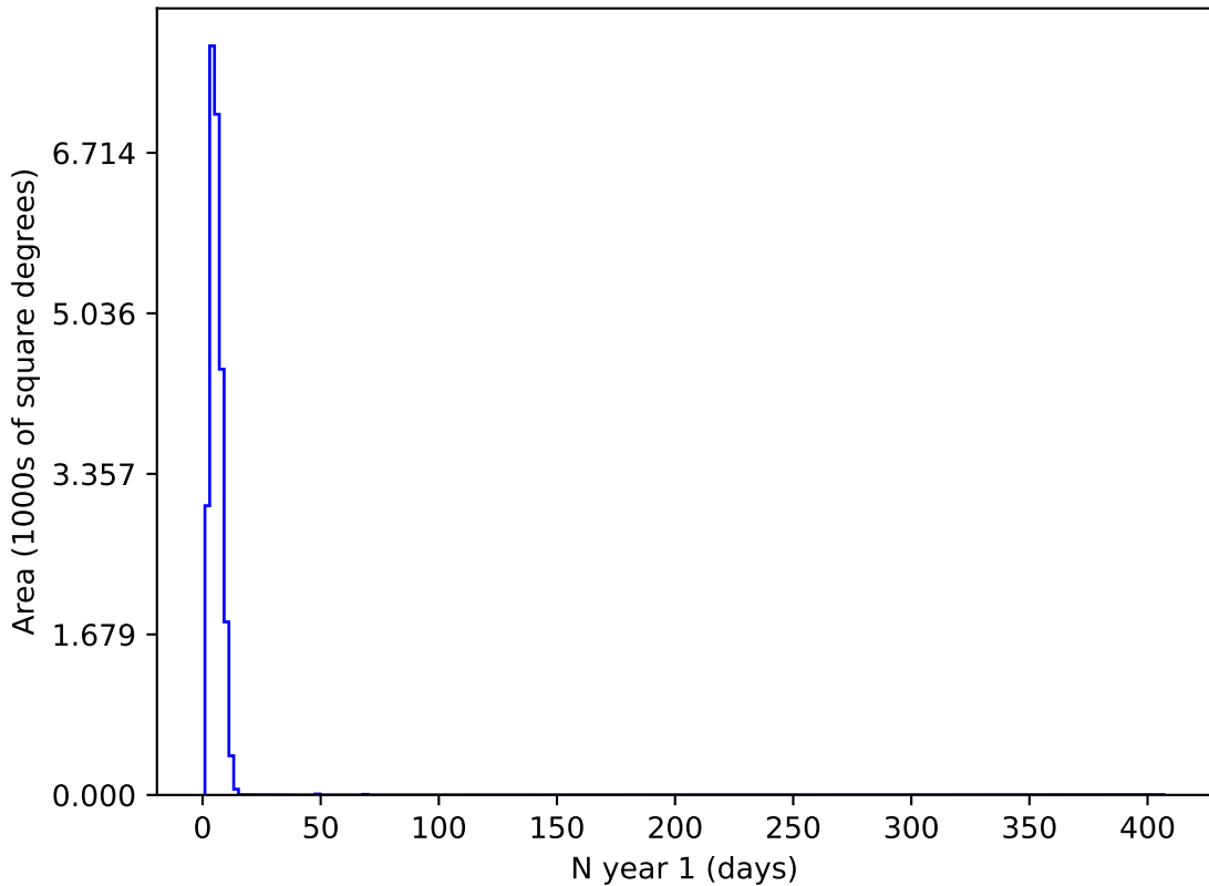
too_10_1v3.4_10yrs u and night < 365: N year 1
