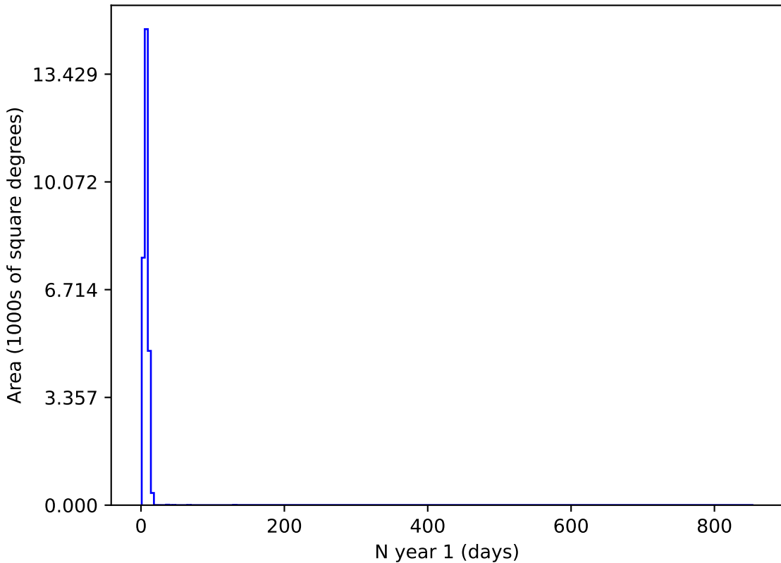
too_10_1v3.4_10yrs g and night < 365: N year 1
