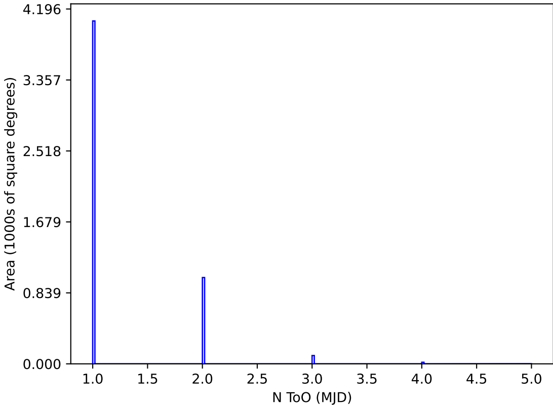
too_10_1v3.4_10yrs z and note like ToO%: N ToO
