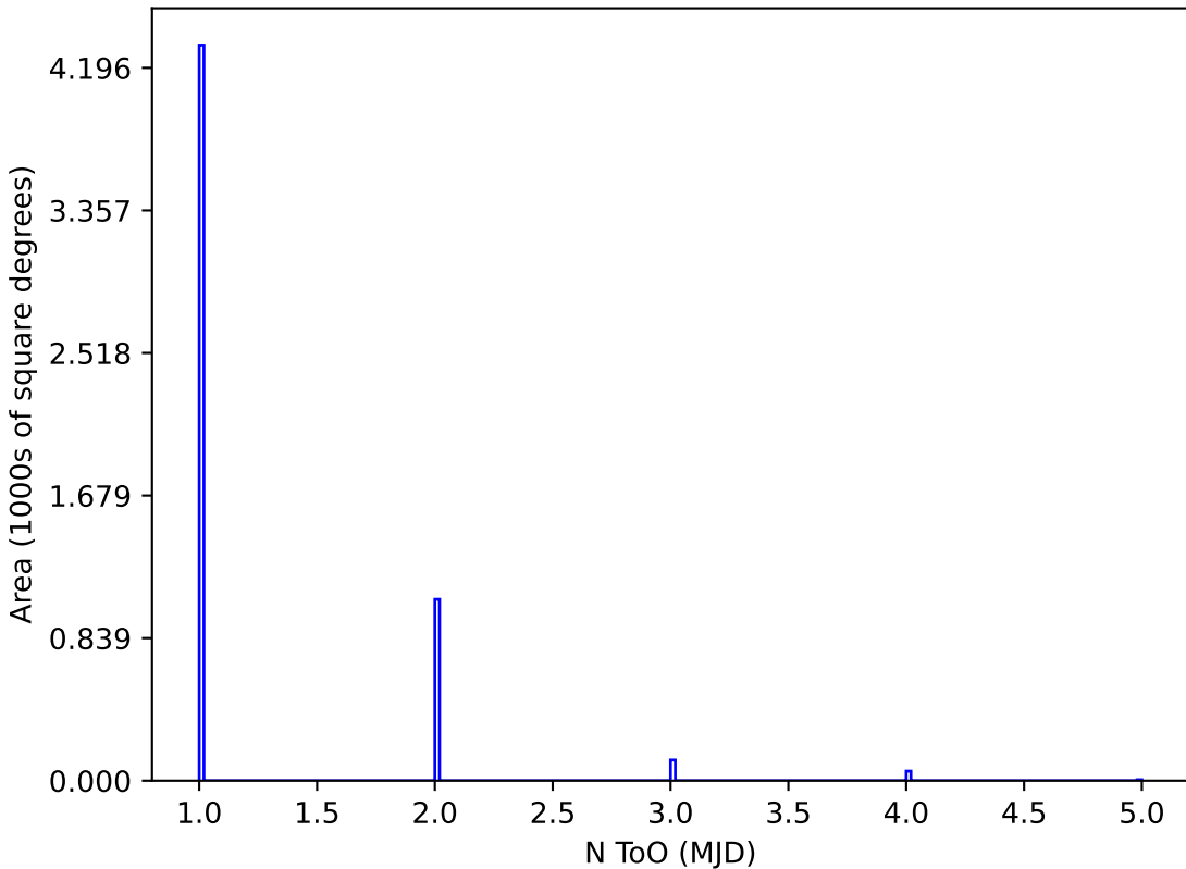
too_10_1v3.4_10yrs g and note like ToO%: N ToO
