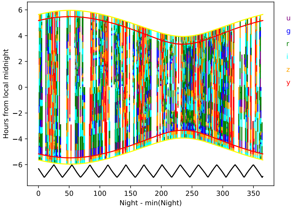
too_10_1v3.4_10yrs year 7-8: Hourglass
