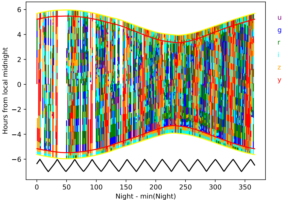
too_10_1v3.4_10yrs year 6-7: Hourglass
