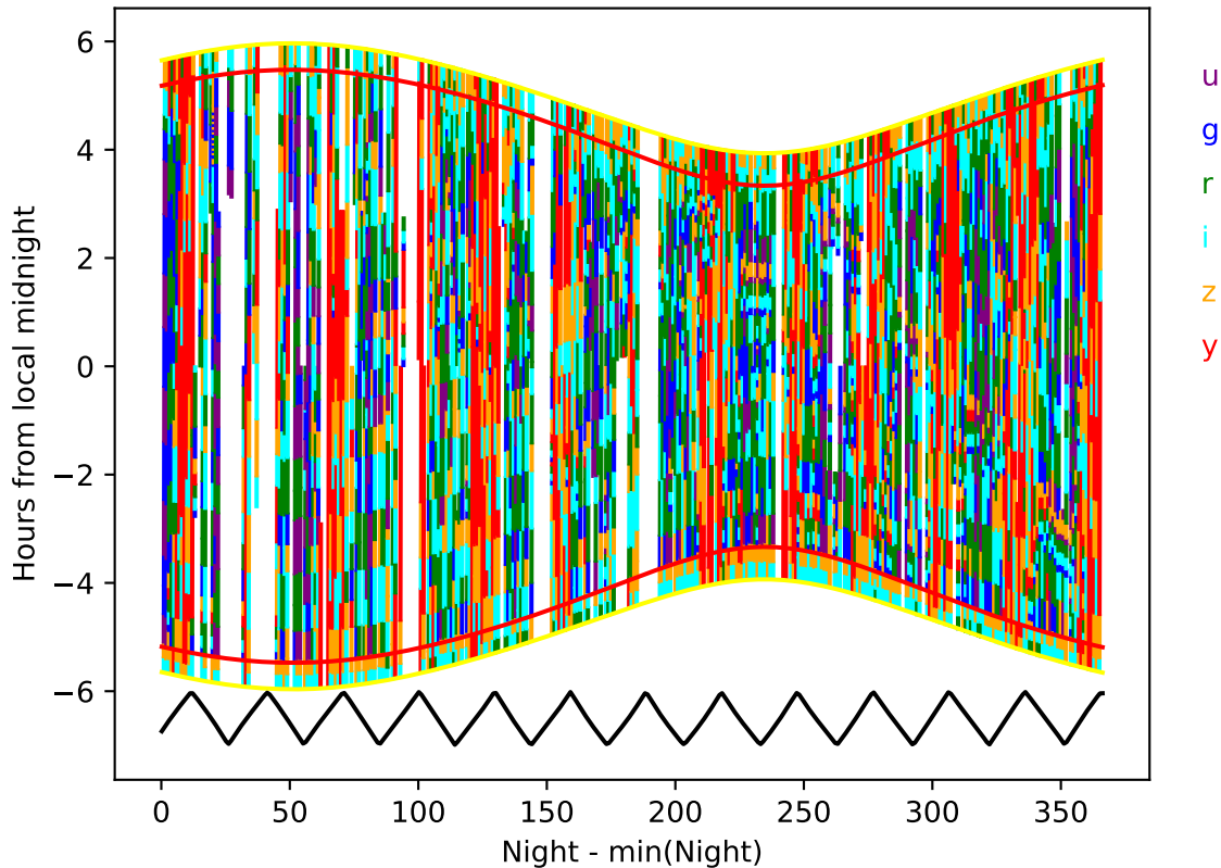
too_10_1v3.4_10yrs year 0-1: Hourglass
