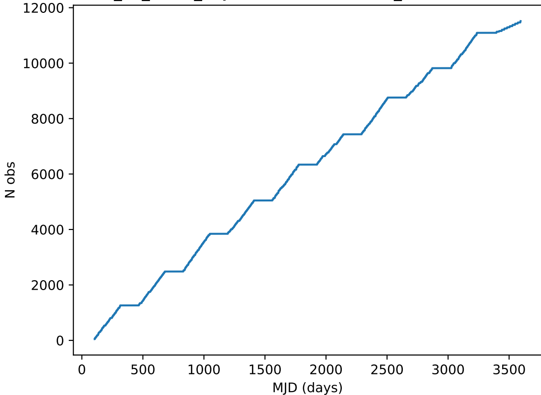
too_10_1v3.4_10yrs note like DD:EDFS_a%: Cumulative
