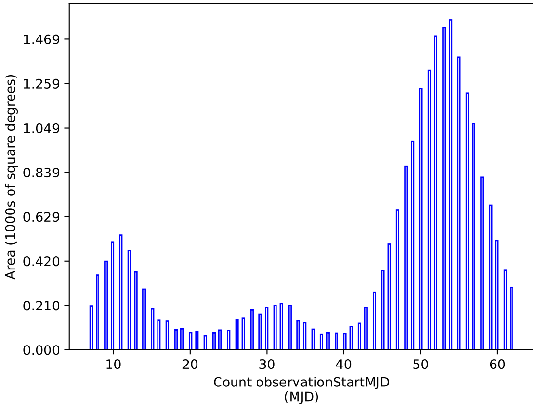
too_10_1v3.4_10yrs u: Count observationStartMJD
