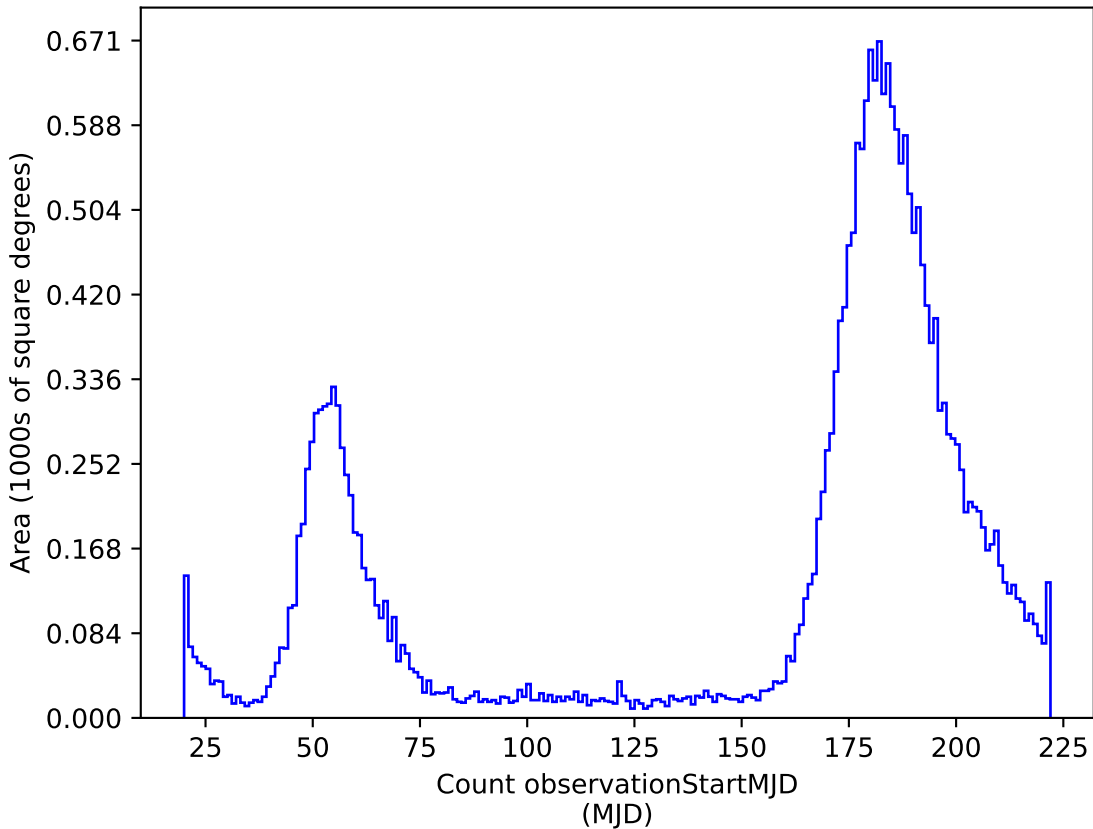
too_10_1v3.4_10yrs r: Count observationStartMJD
